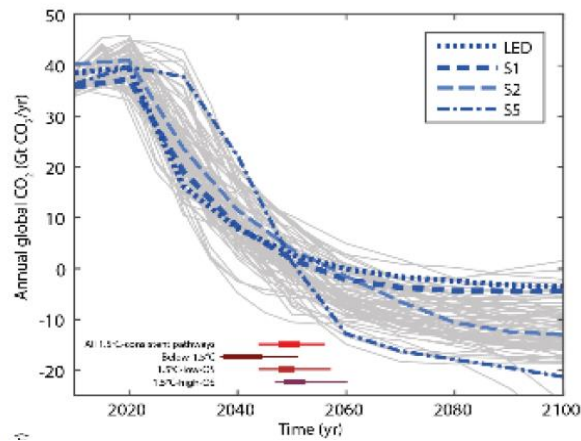
Figure 14: Global net CO 2 emissions in Below-1.5°C, 1.5°C-low-OS, and 1.5°C-high-OS pathways with archetype scenarios highlighted 30
