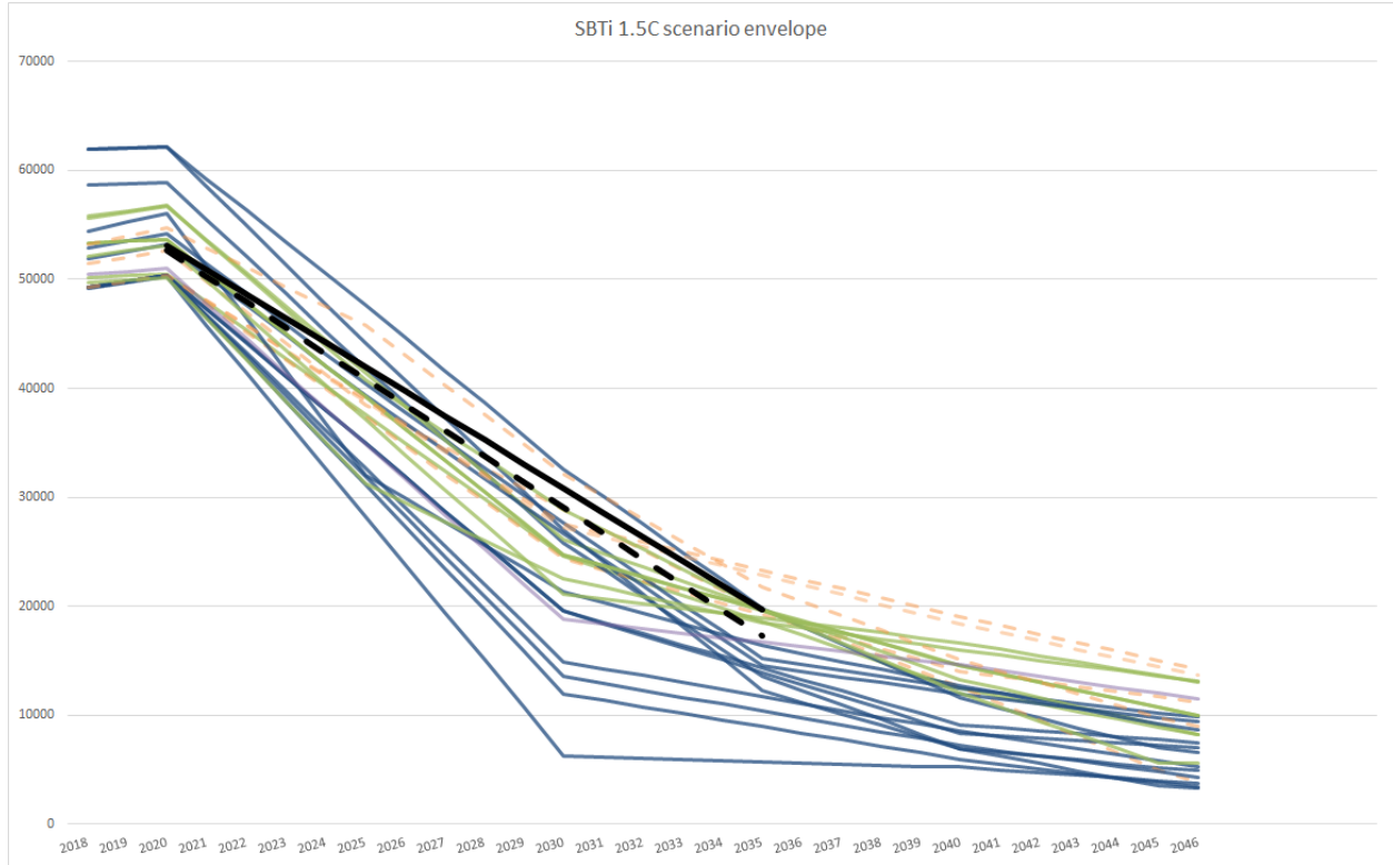
Figure 5: Scenarios in final 1.5°C envelope are shown by navy, green, and violet lines, colored by linear reduction between 2020-2035 (navy: higher than median; green: lower than median; violet: pre-screen median; where pre-screen median refers to the scenario envelope before the bottom 20th percentile has been removed). Dotted orange lines are the bottom 20th percentile scenarios, which are removed by the qualitative screen. Dotted black line shows a hypothetical scenario where emissions are reduced at the pre-screen envelope median (4.5% linear), while solid black line shows emissions reduced at the post-envelope minimum (4.2% linear)
