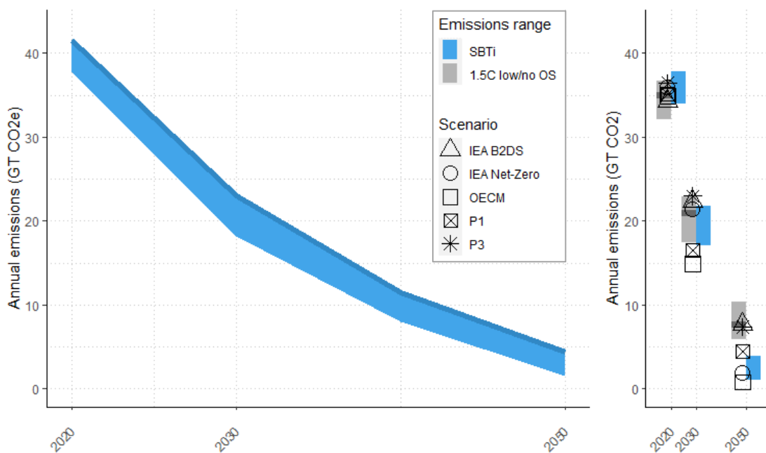
Figure 2. SBTi emissions corridors (light blue) for a. cross-sector GHG emissions and b. CO 2 only with comparison to the median (dark grey line) and interquartile range of 1.5°C low/no overshoot scenarios (grey bars) and individual scenarios (black icons). GHG emissions from forestry, land-use, and agriculture; landfill waste; and fluorinated gases are excluded from both corridors. The SBTi's cross-sector emissions pathway (dark blue line), used to define the minimum ambition of many SBTs, is based on the upper bound of the cross-sector GHG emissions corridor
