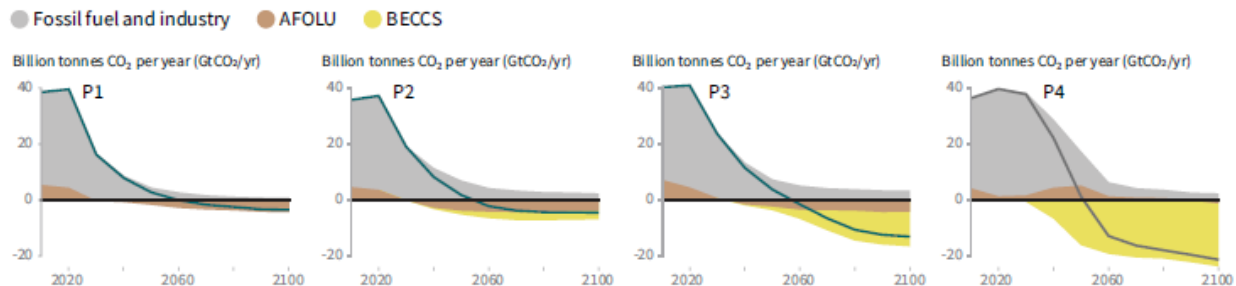
Figure 1: Global net CO 2 emissions in the low/no-overshoot 1.5°C set (grey) with archetype scenarios in blue (top) and breakdown of contributions to global net CO 2 emissions in four archetype scenarios (bottom).
