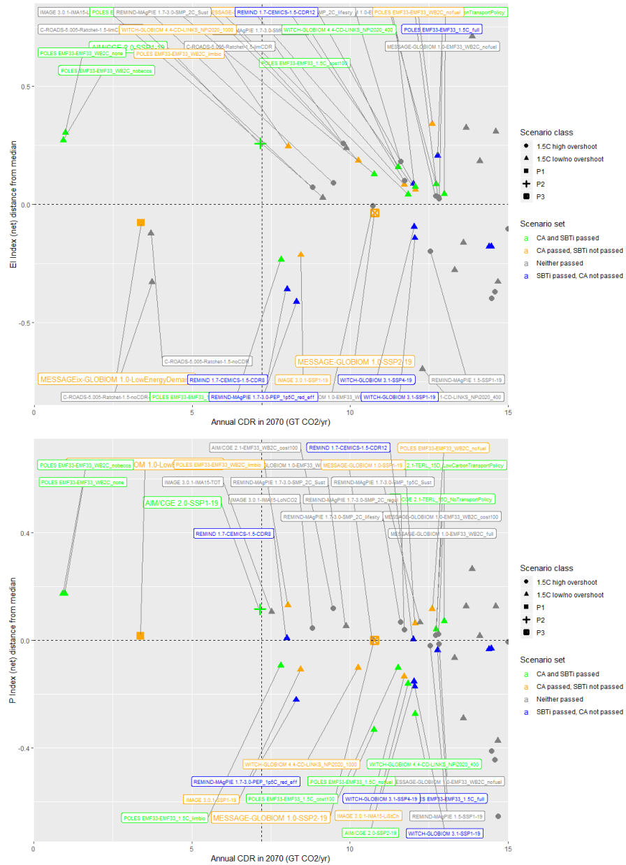
Figure 21: EI Index relative to 1.5C low/no-overshoot set median (average of 2030, 2040 and 2050) vs CDR with model-scenario labels (top). P Index relative to 1.5C low/no-overshoot set median (average of 2030, 2040, and 2050) vs CDR with model-scenario labels (bottom). Chart is divided into quadrants where the vertical line demarcates scenarios with over/under 7.2 GT CO 2 /year and the horizontal line demarcates scenarios with EI Indices over/under the 1.5C low/no-overshoot median in the given year. Scenarios with >15 GT CDR/yr are not shown.
