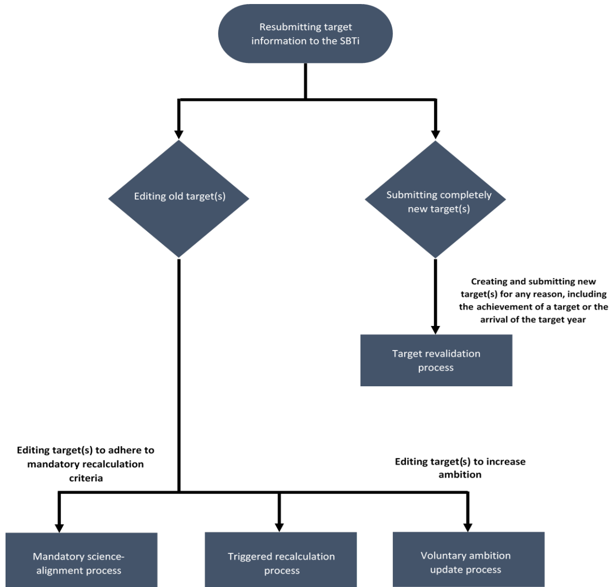
Figure 4. Recalculation process
